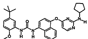
1-(5-tert-Butyl-2-methoxy-phenyl)-3-[4-(2-cyclopentylamino-pyrimidin-4-yloxy)-naphthalen-1-yl]-urea;
